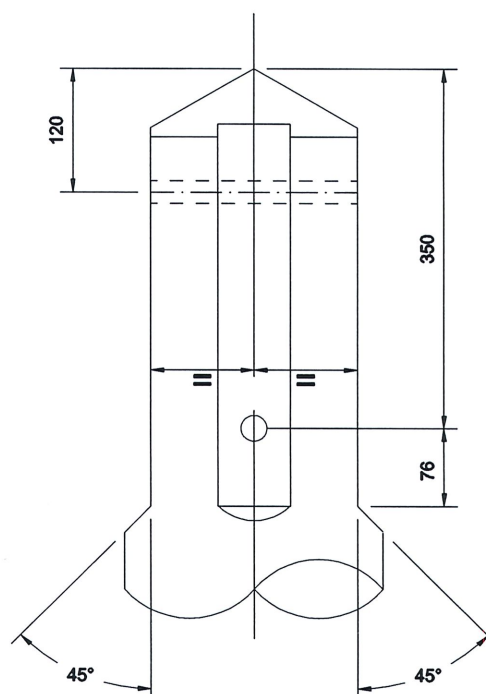
SIDE ELEVATION ON VIEW 'A' & 'B' SCALE 1:5
